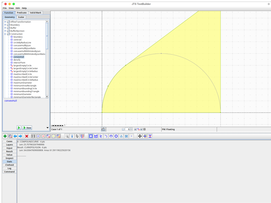
TS-6. Compound H-CC hull area 61.59119, CurvePolygon with CircularString.
